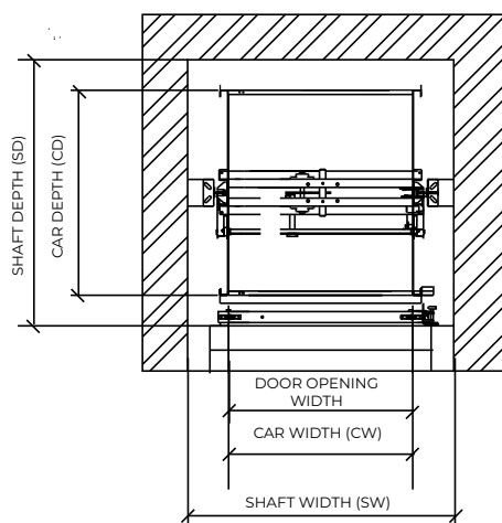
GENERAL SHAFT LAYOUT - INLINE ENTRANCES
