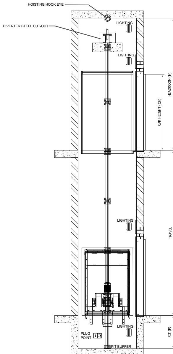
SECTIONAL VIEW OF MR BELOW ADJACENT SHAFT - INLINE ENTRANCES
