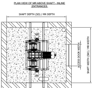
MRA (Machine Room Above)
