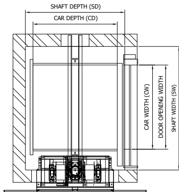
PLAN VIEW OF MR BELOW ADJACENT SHAFT - INLINE ENTRANCES
