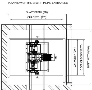
MRL (Machine Room Less)
